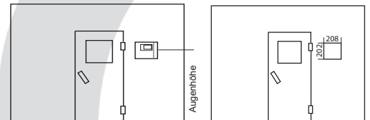
Cut-out size for control panel
